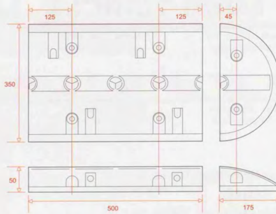
ECORAMP4 Each section 500mm long. Sold in pairs 1 Yellow and 1 Black
